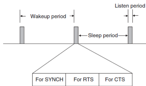
Figure 5.6 S-MAC principle
